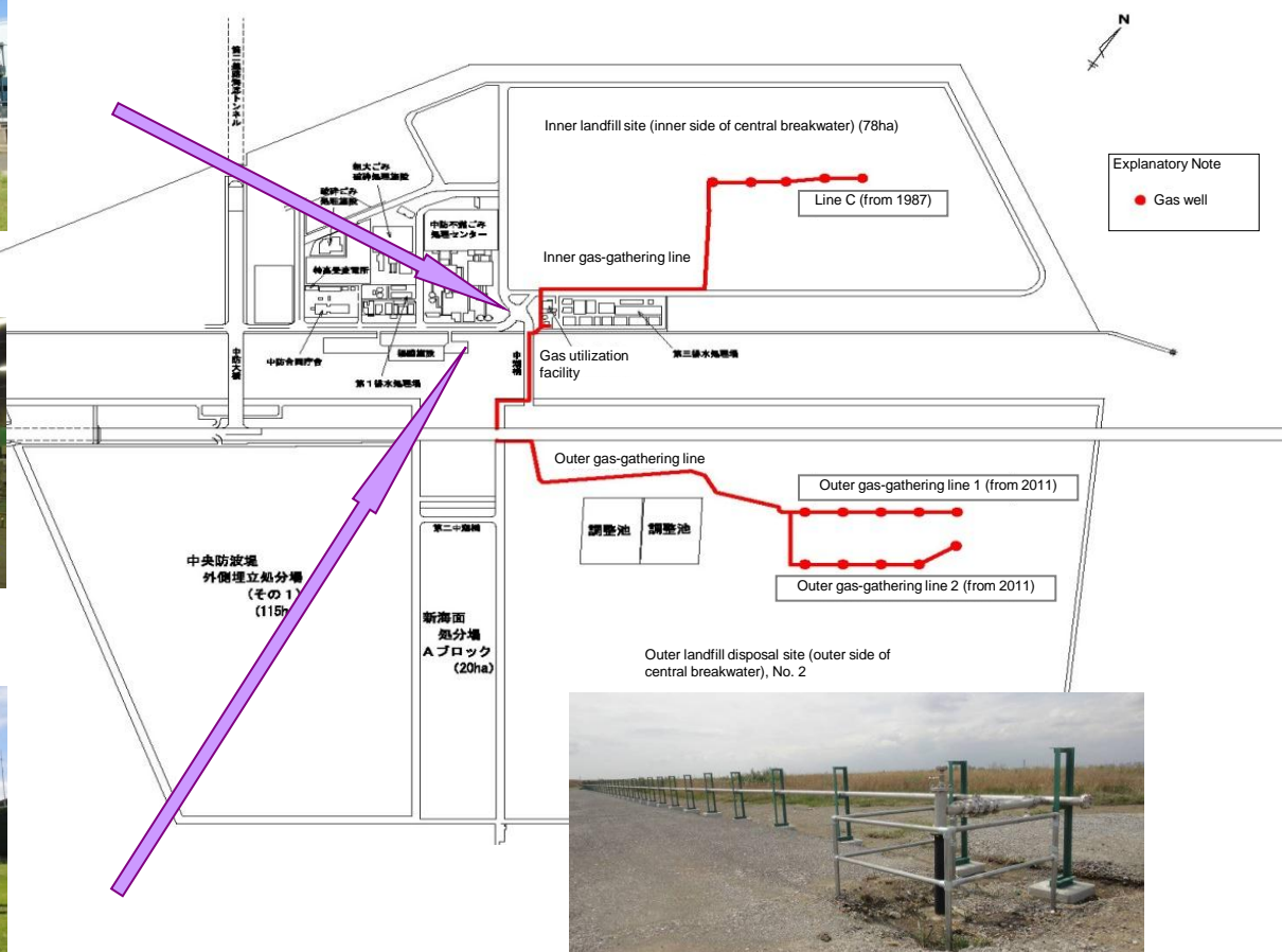
Outer gas-gathering line
